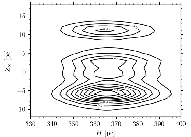
Fig. 15. Posterior probability density for the scale height H and solar z coordinate with respect to the Galactic plane inferred from the hierarchical Bayesian model.
