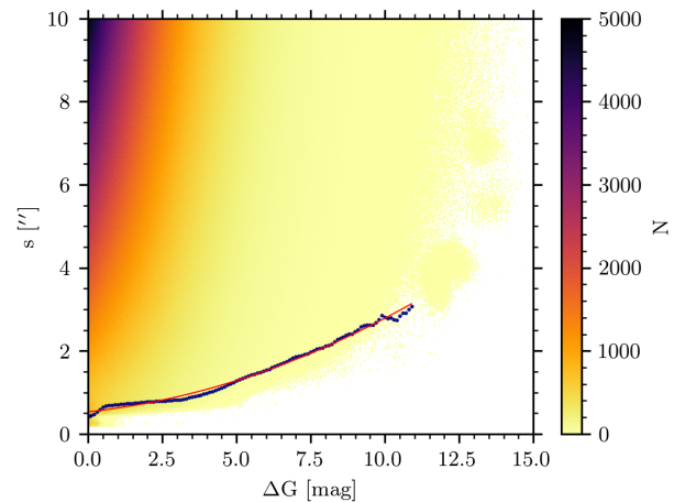
Fig. 8. Magnitude difference, \Delta G , vs. angular separation, s , of all objects in Gaia EDR3 colour-coded by density in [0.02, 0.02] bins. The blue points represent the 99.5 percentiles of the separations, and the red line is a fit to these values and is reported in Eq. 2.
